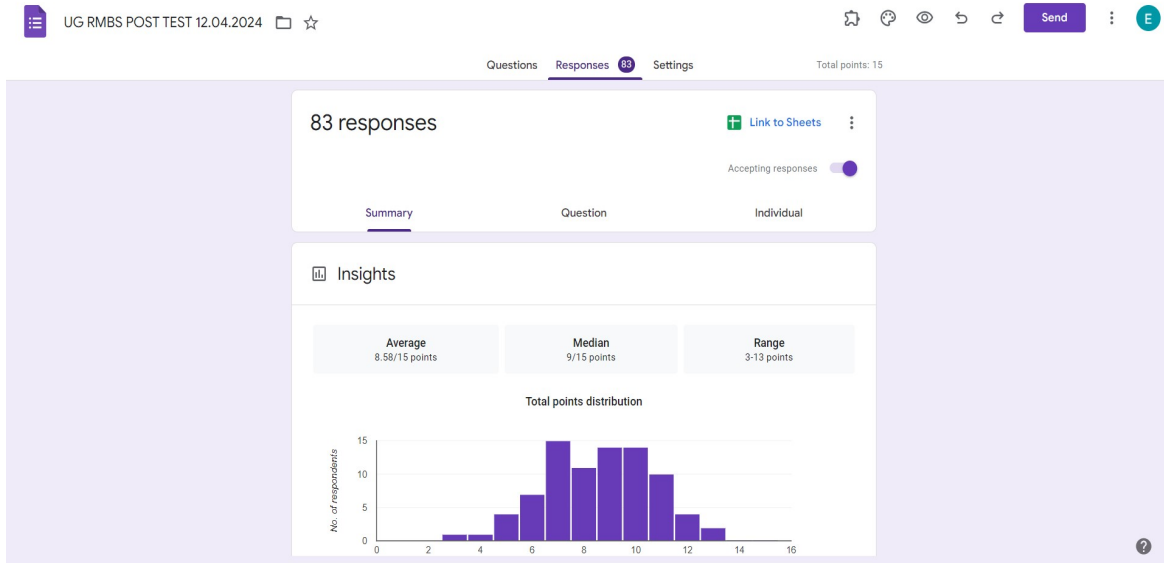
Figure 2: Post-test Score
