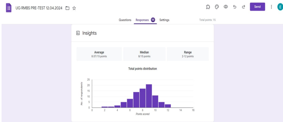
Figure 1: Pre-test Score
